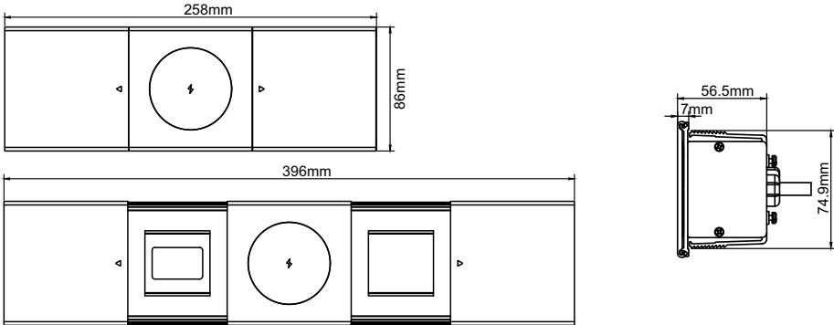
STS-SC04/2F/Qi 2 modules unit
